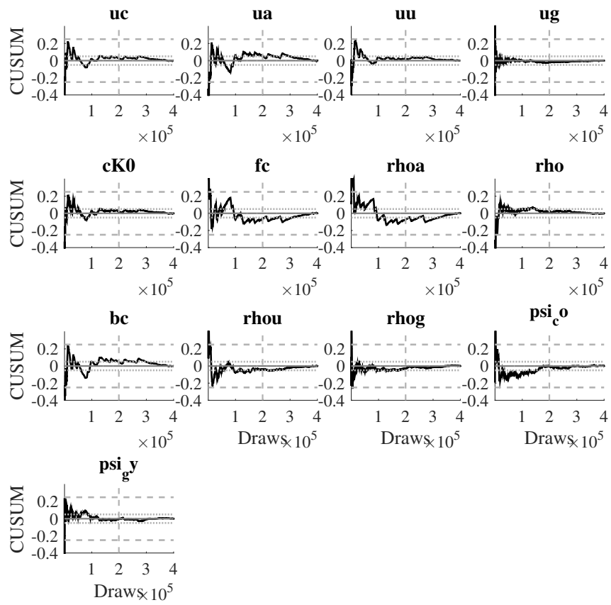
Figure 8: CUSUM statistics.
