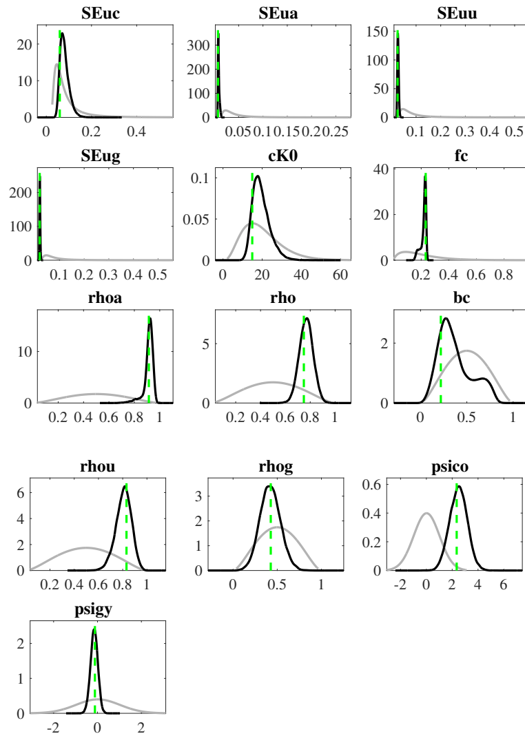
Figure 7: Prior (grey) and posterior (black) distributions.
