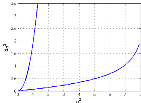
Figure 4: The Admissible Volatility Step Size
