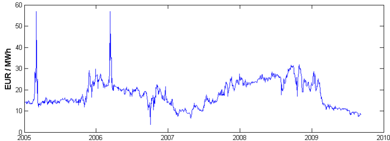
Figure 2: The TTF Day-Ahead Price
